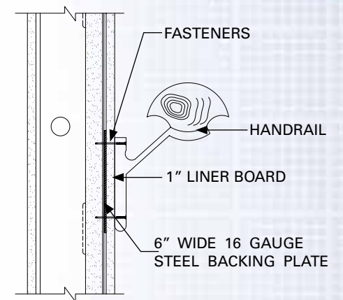
12 HANDRAIL CONNECTION
