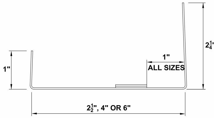
TABBED TRACK
