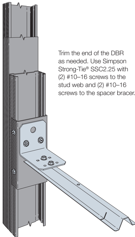
DBR End-of-Run for 2.5" Studs with SSC2.25
