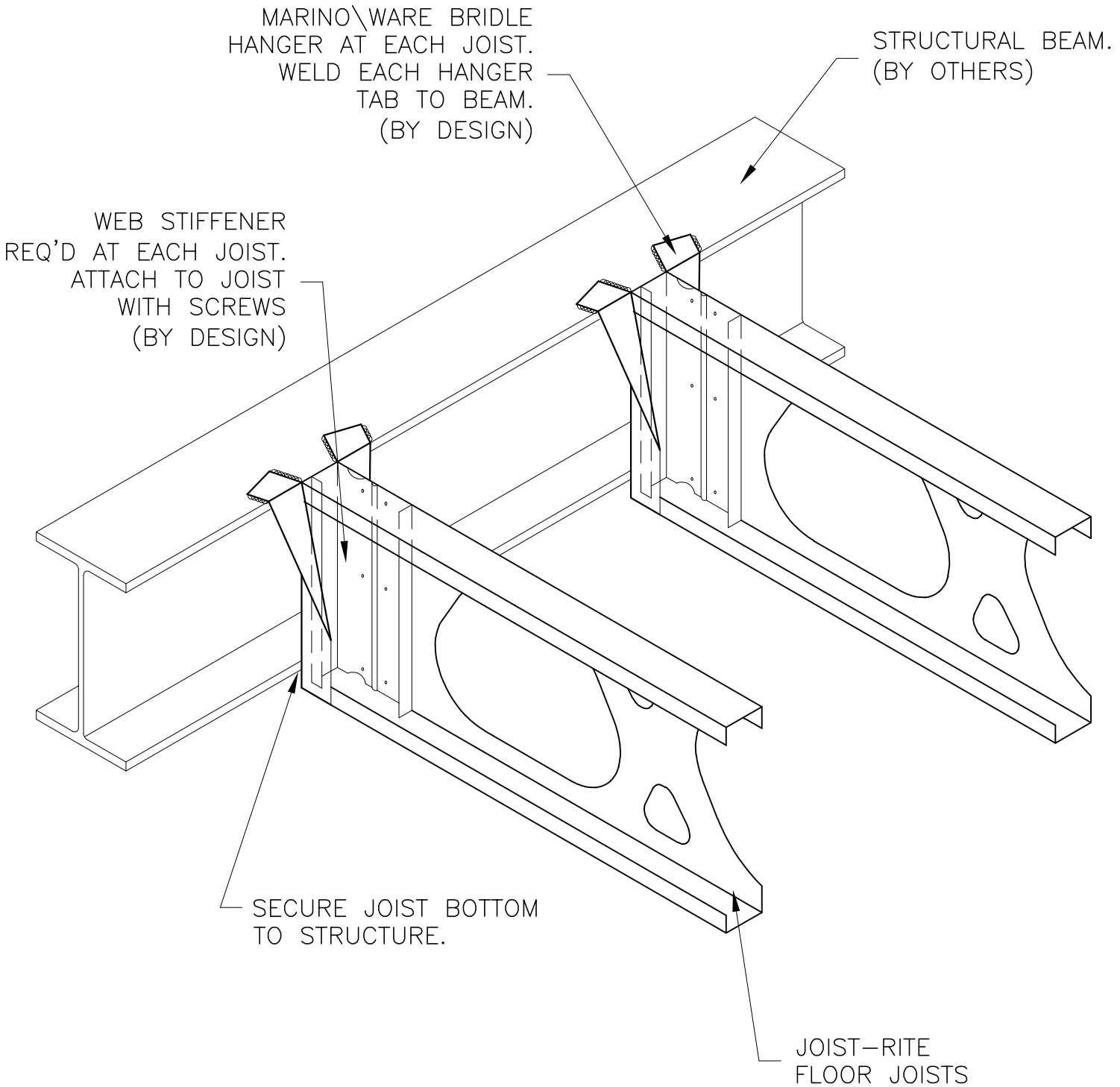
JOIST CONNECTION TO I-BEAM USING MARINO\WARE BRIDLE HANGER
