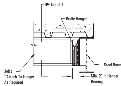
JOIST @ STEEL BEAM W/BRIDLE HANGER
