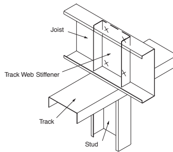
WEB STIFFENER: TRACK INSIDE JOIST
