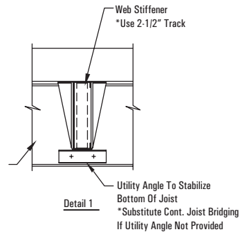
JOIST @ STEEL BEAM W/BRIDLE HANGER
