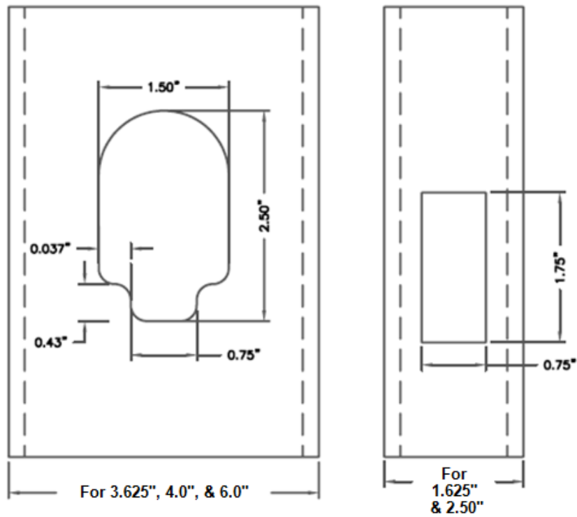
Figure 2 – ViperStud Knockouts
