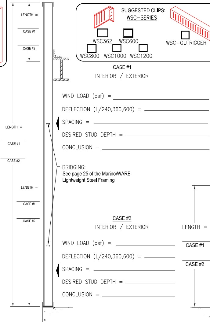
CURTAIN WALL (BY-PASS)
