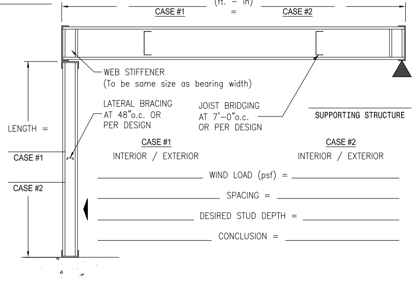
BEARING WALL
